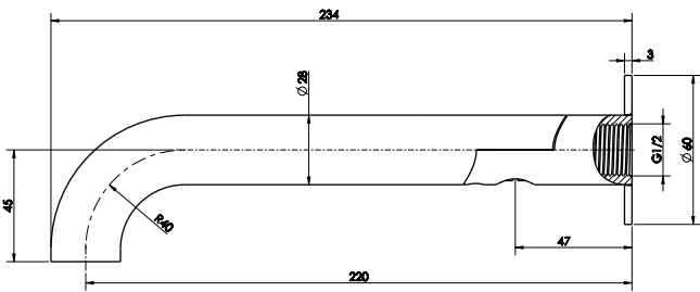
① Dimensional Drawing of Spout
